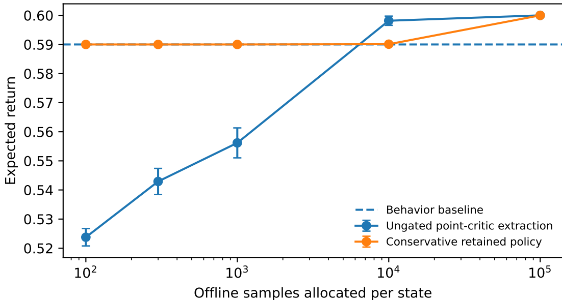
Estimation-only control ( K = 32 )
