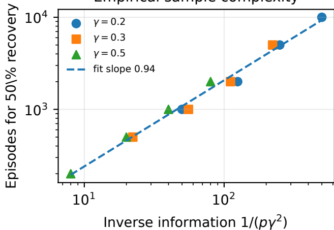
Empirical sample complexity
