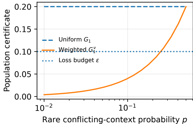
Uniform vs. deployment-weighted
