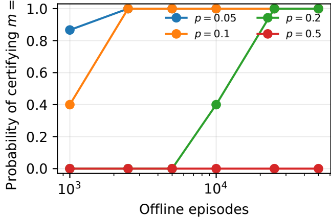
Finite-sample weighted selection
