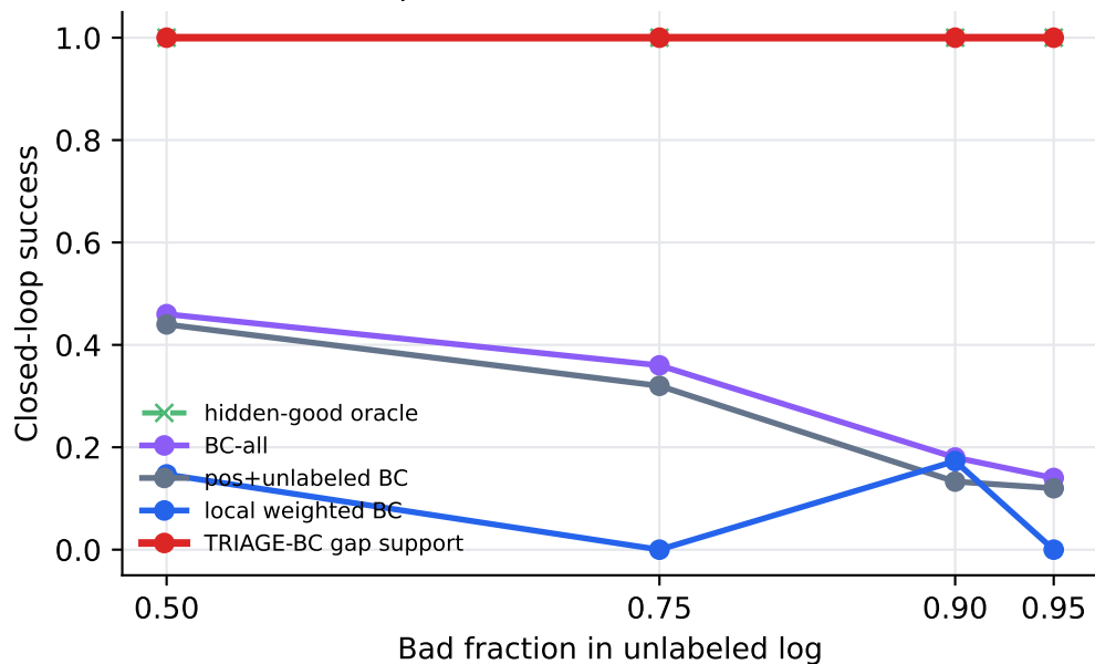
Equal scarce labels: n_+ = n_- = 2
