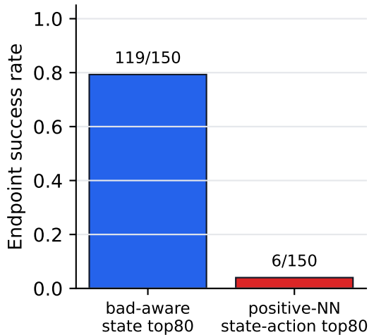
Policy endpoint
