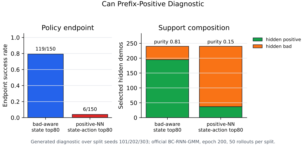
Figure 8: Generated Can prefix-positive diagnostic over split seeds 101/202/303. Explicit failures let the bad-aware selector recover far cleaner full-trajectory support and transfer to the BC-RNN-GMM endpoint, but this remains a generated diagnostic rather than a primary benchmark row.
