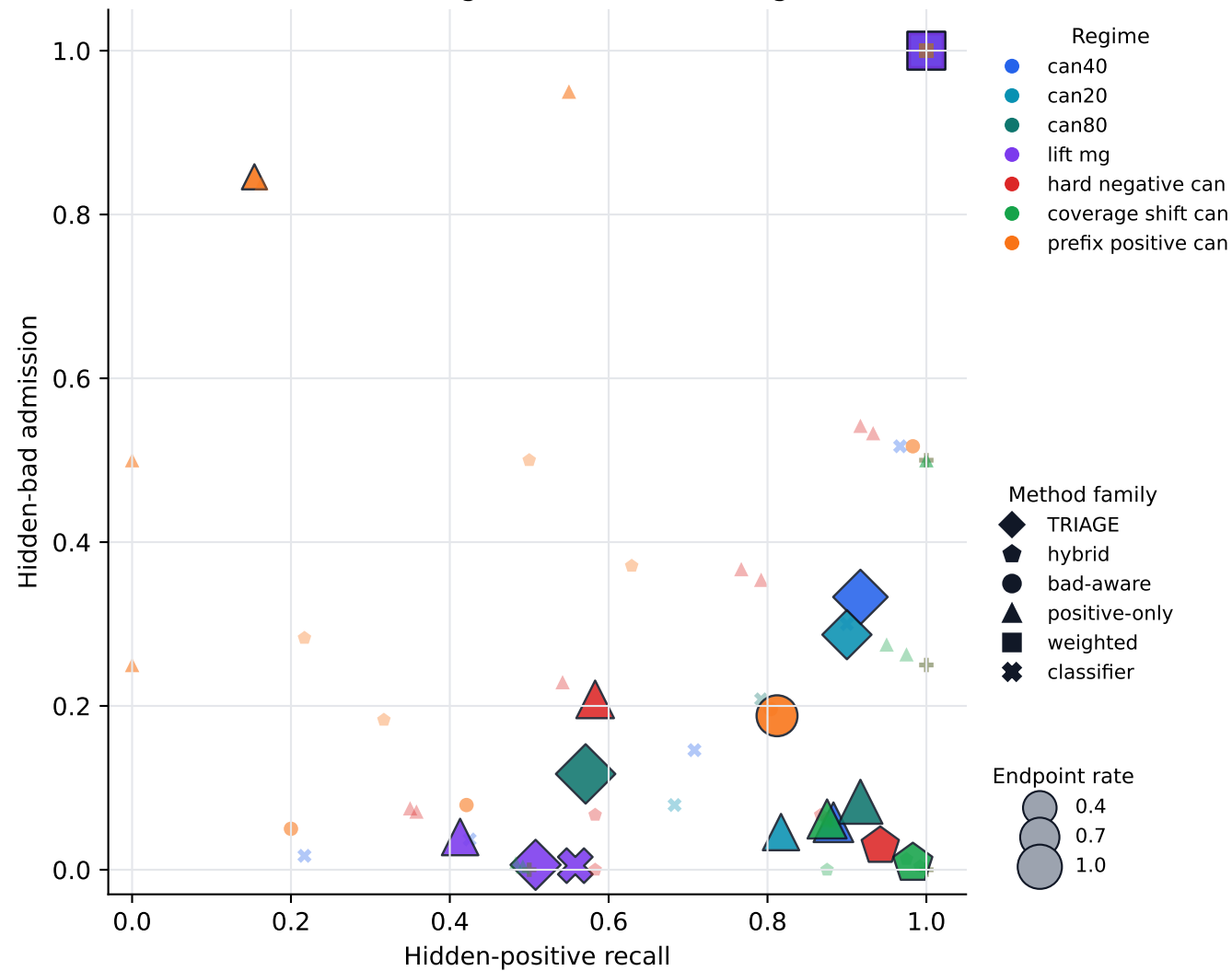
Precision/Coverage Frontier Across Regimes
