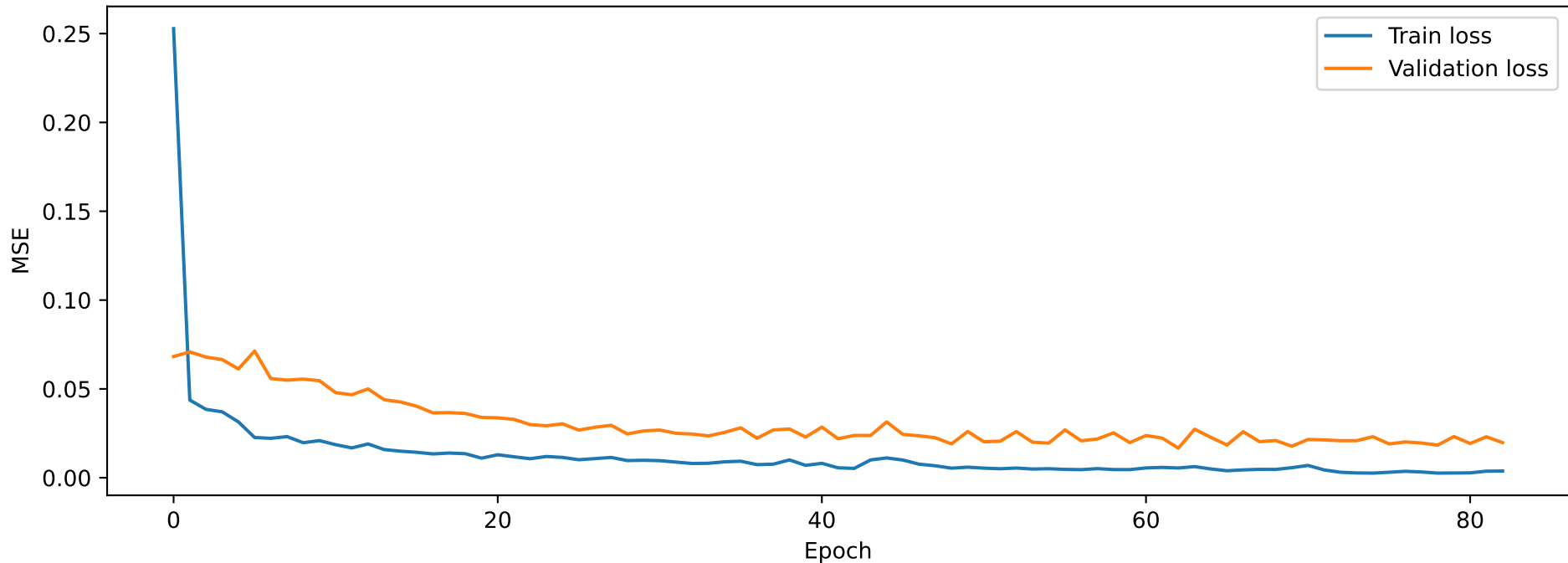
Okayama - Training Curve
