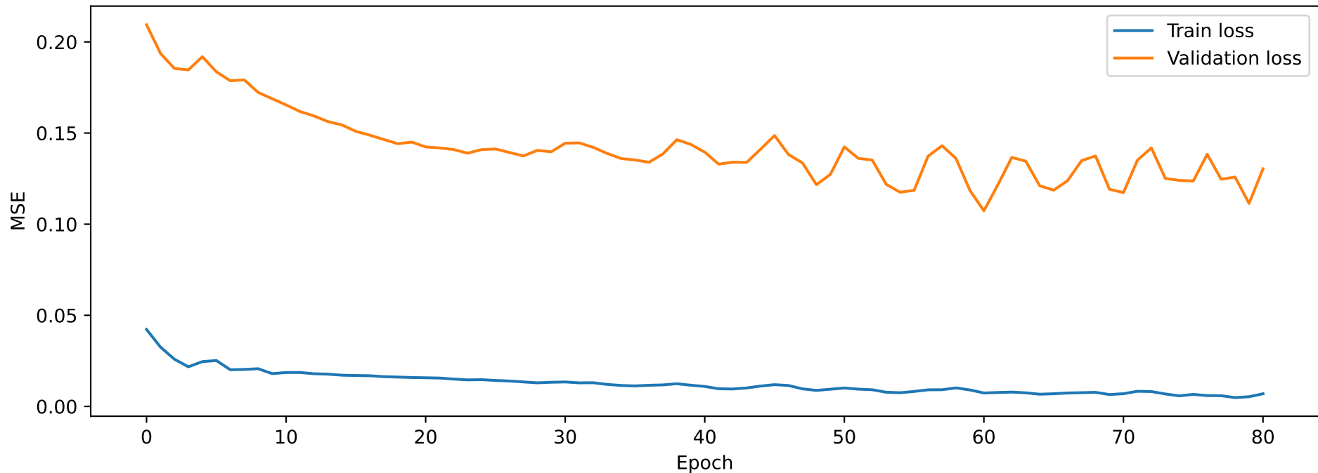
Saga - Training Curve
