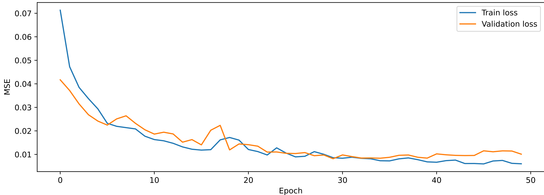
Aichi - Training Curve
