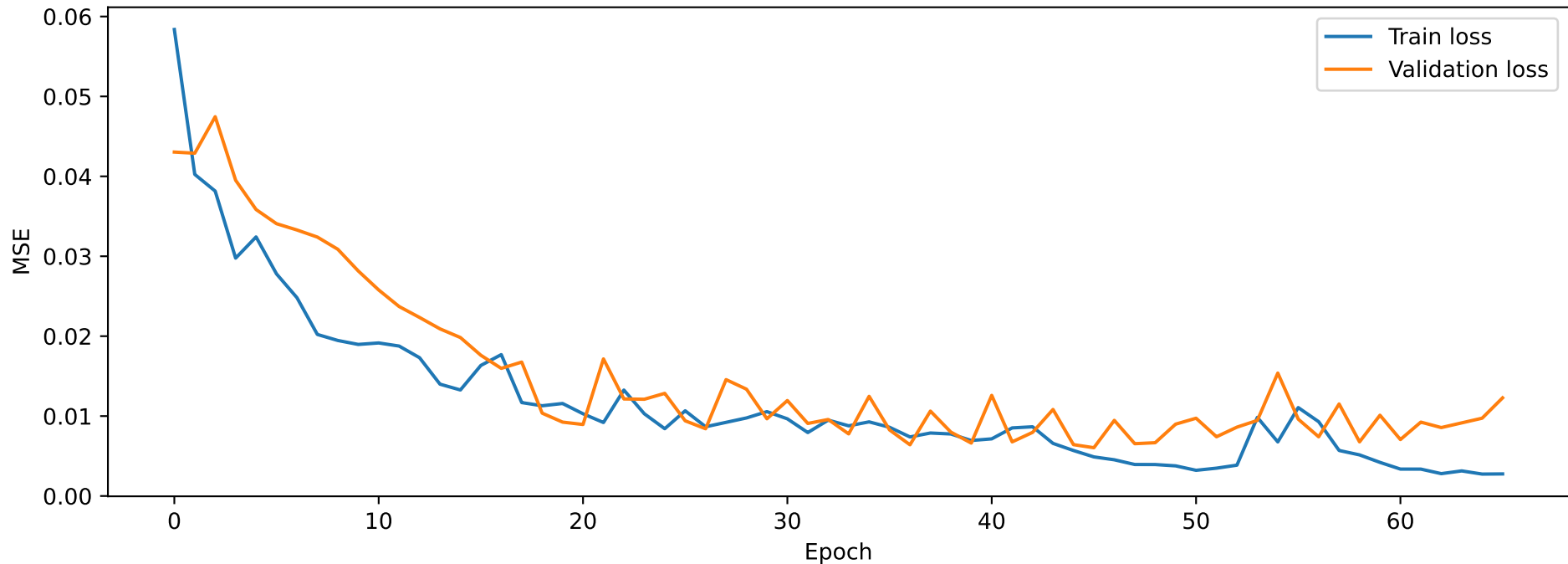
Kanagawa - Training Curve
