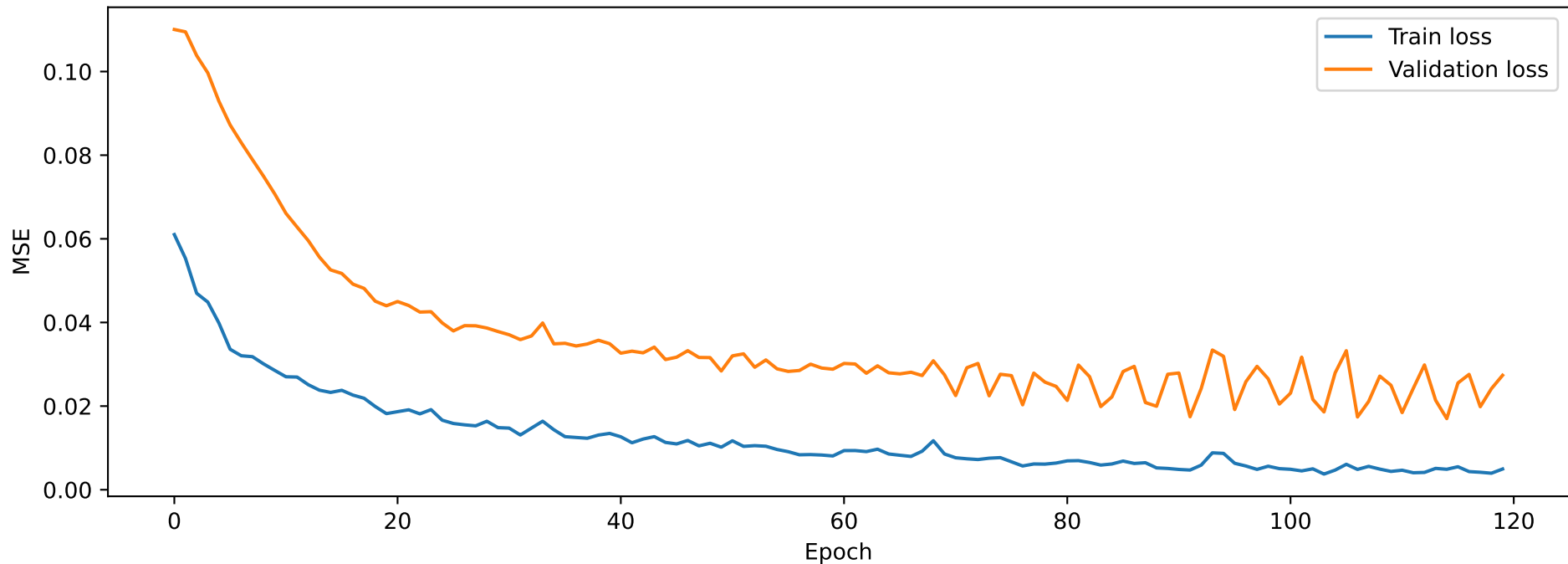
Oita - Training Curve
