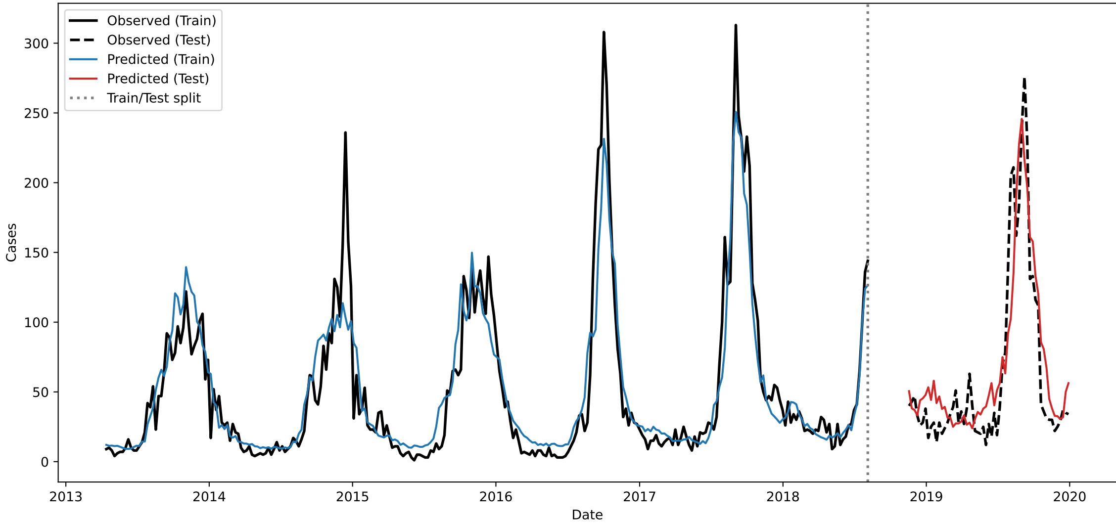
Chiba - Fit (Original Scale)
