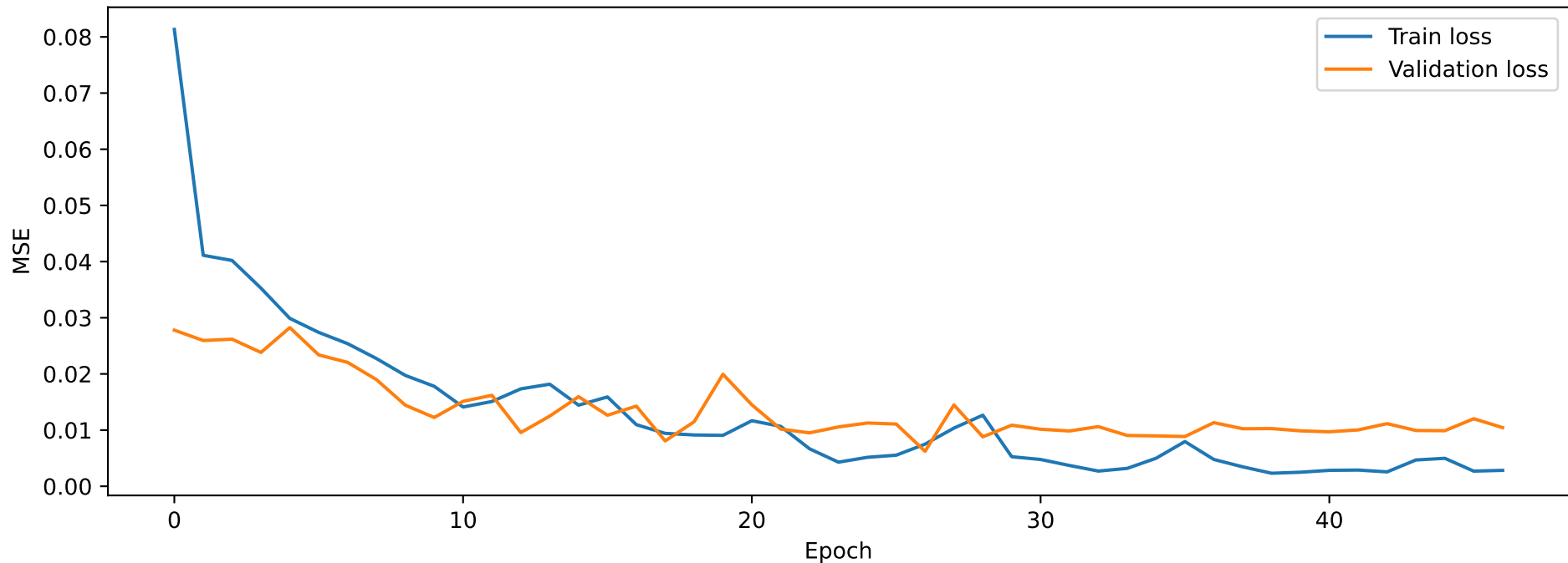
Ibaraki - Training Curve
