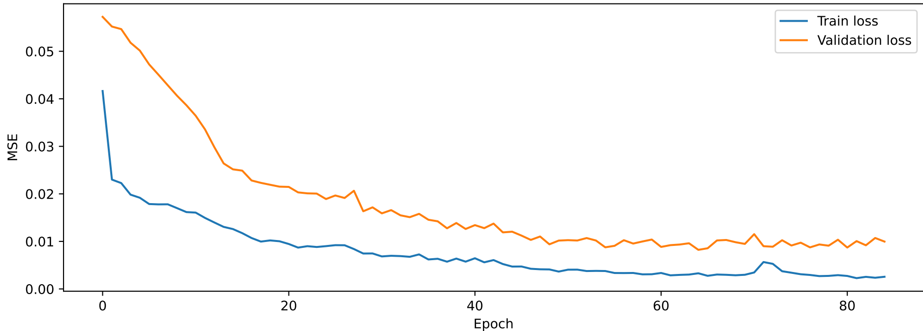
Kagoshima - Training Curve
