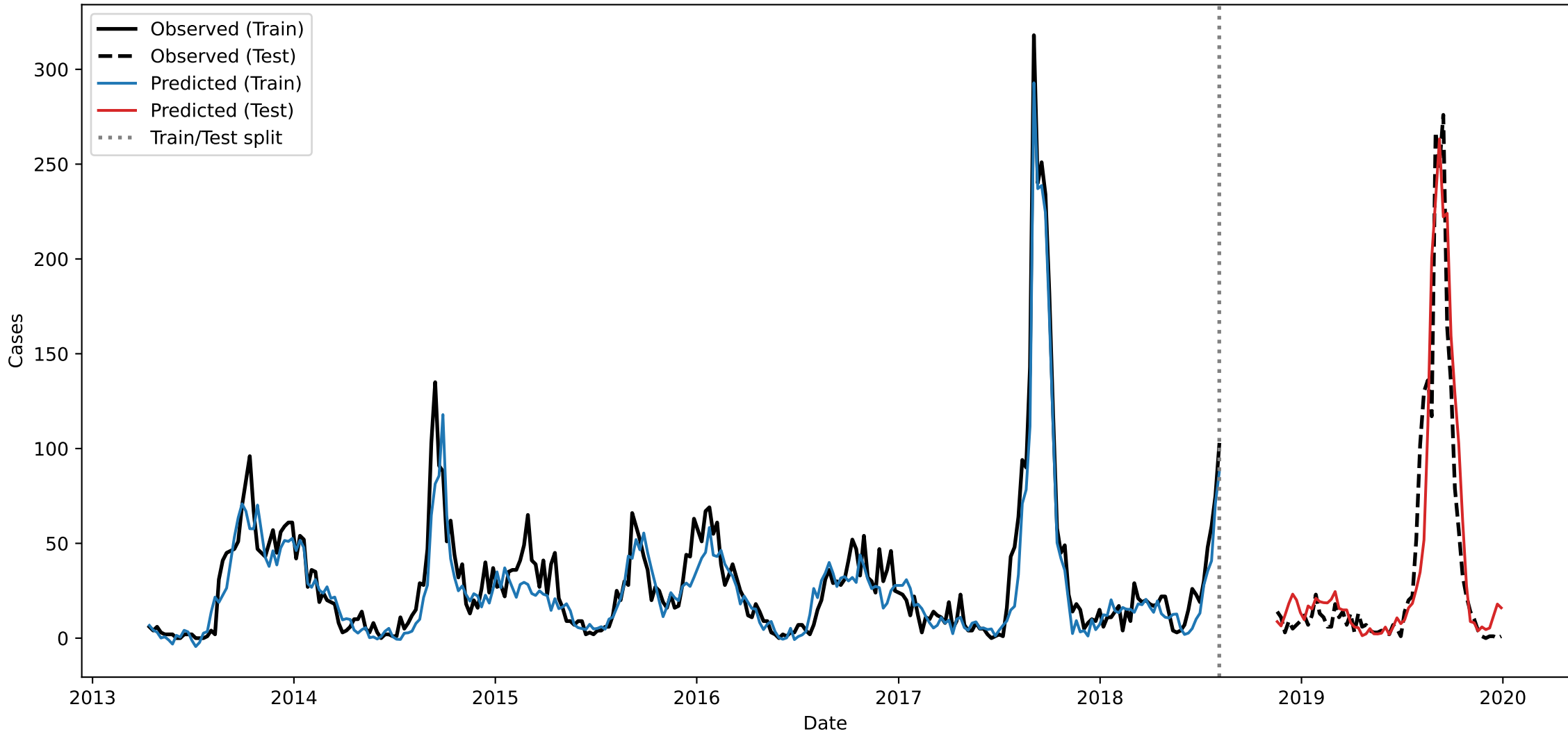
Nagasaki - Fit (Original Scale)
