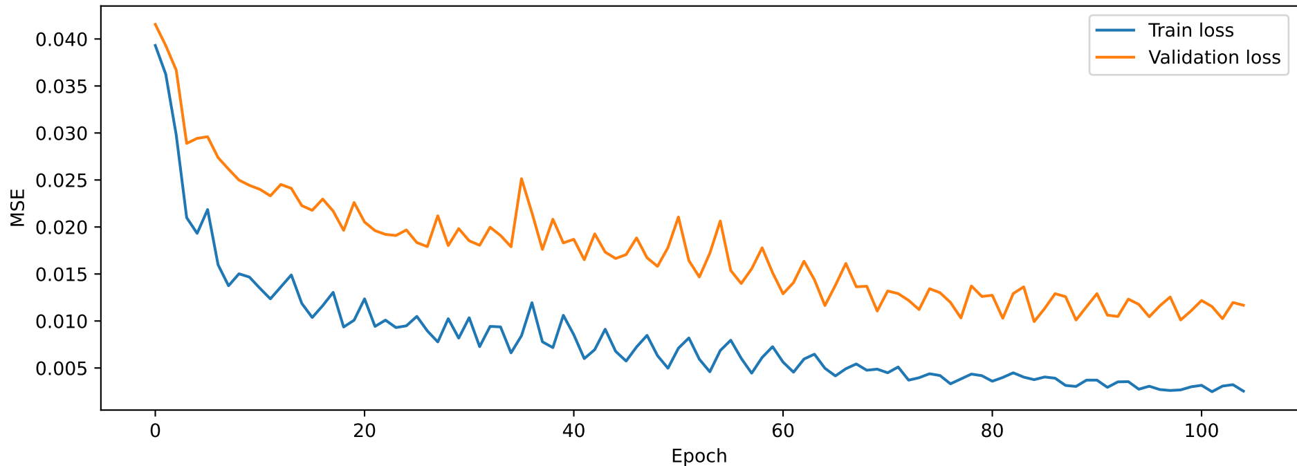
Niigata - Training Curve
