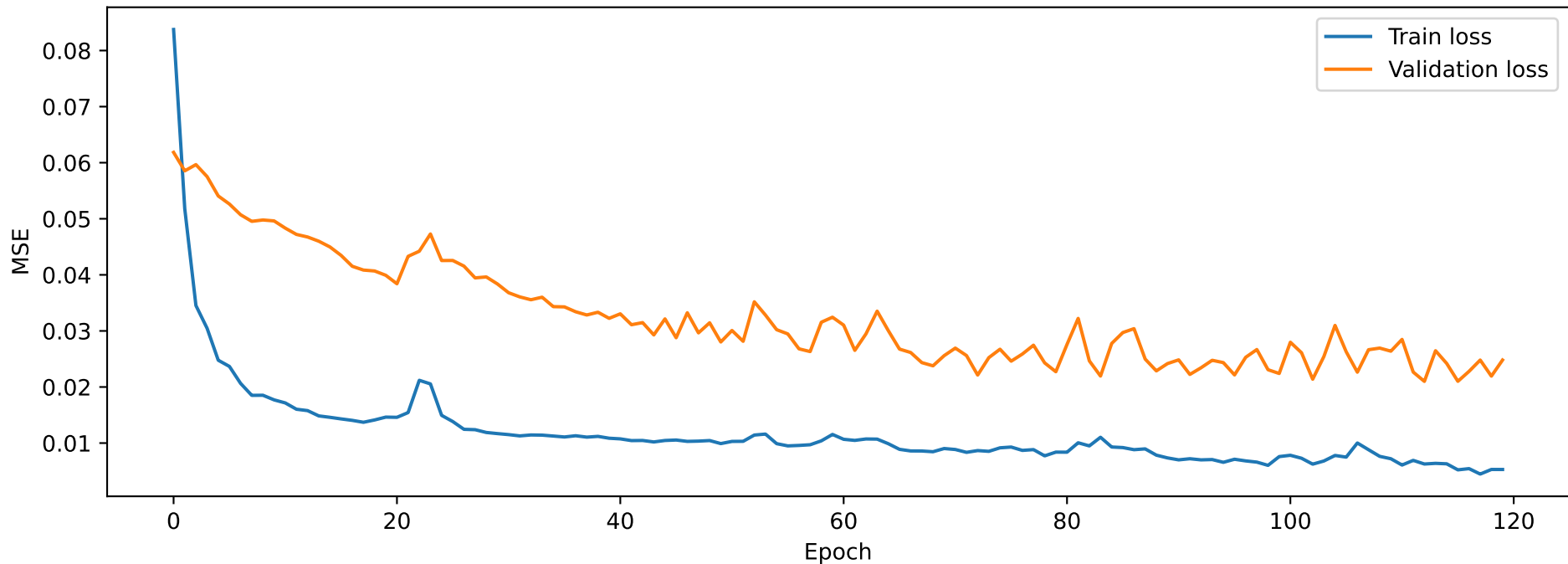
Nara - Training Curve
