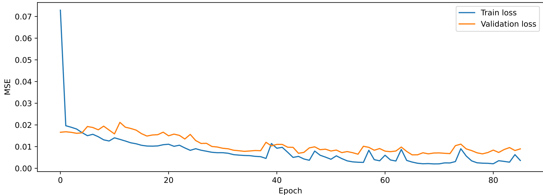
Kochi - Training Curve
