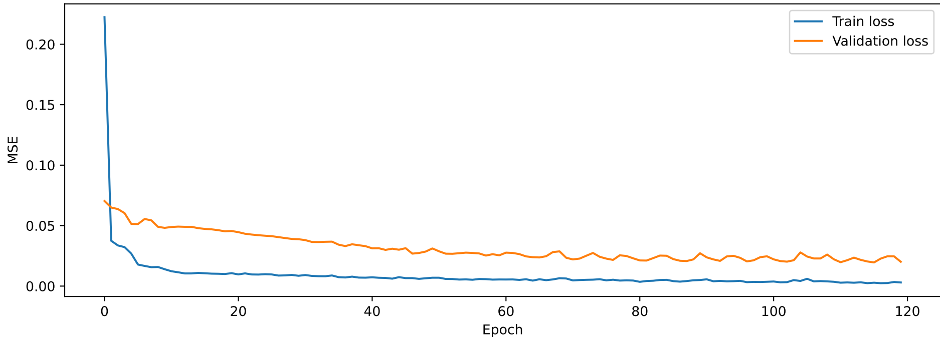
Hiroshima - Training Curve
