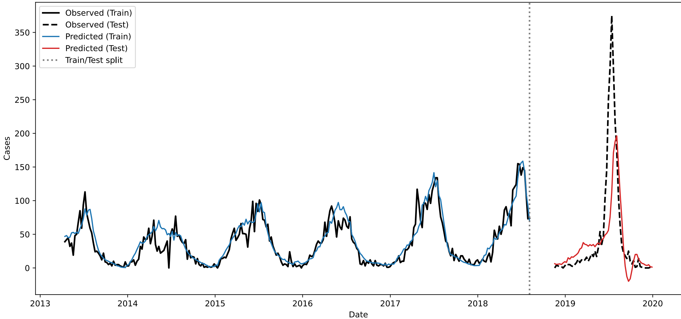
Okinawa - Fit (Original Scale)
