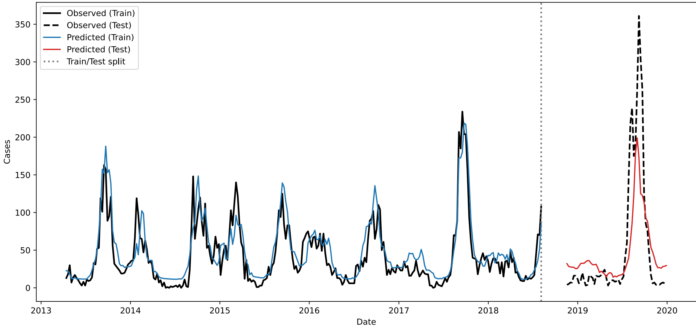
Miyazaki - Fit (Original Scale)
