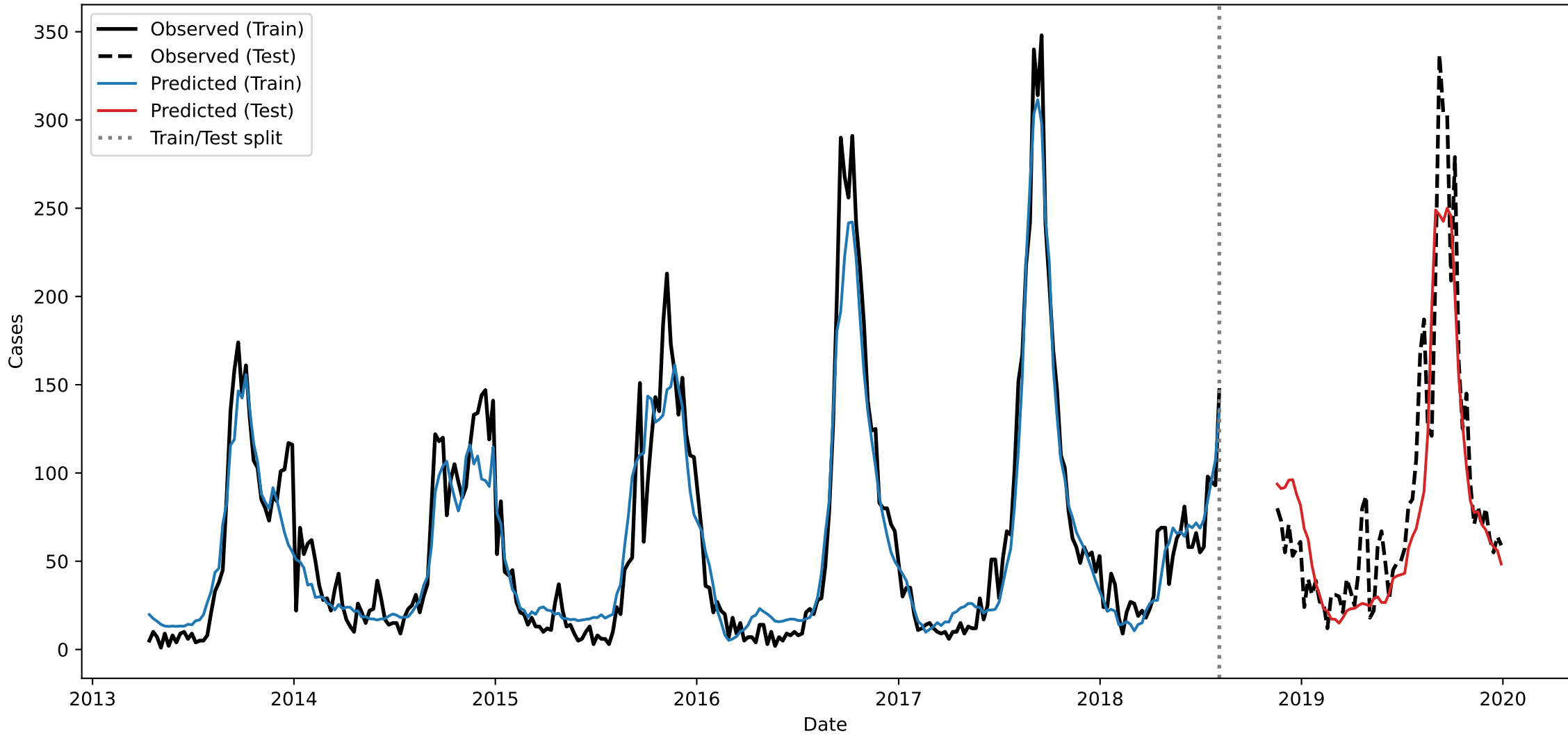
Niigata - Fit (Original Scale)
