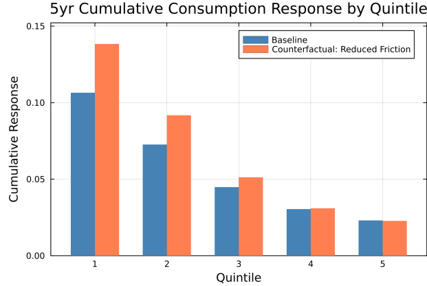
Figure 16: Consumption Response Decomposition: Baseline vs. Reduced Frictions
