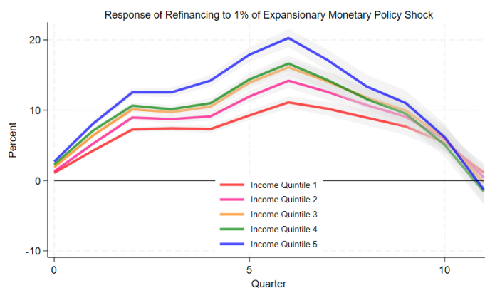
(a) Equation 25
