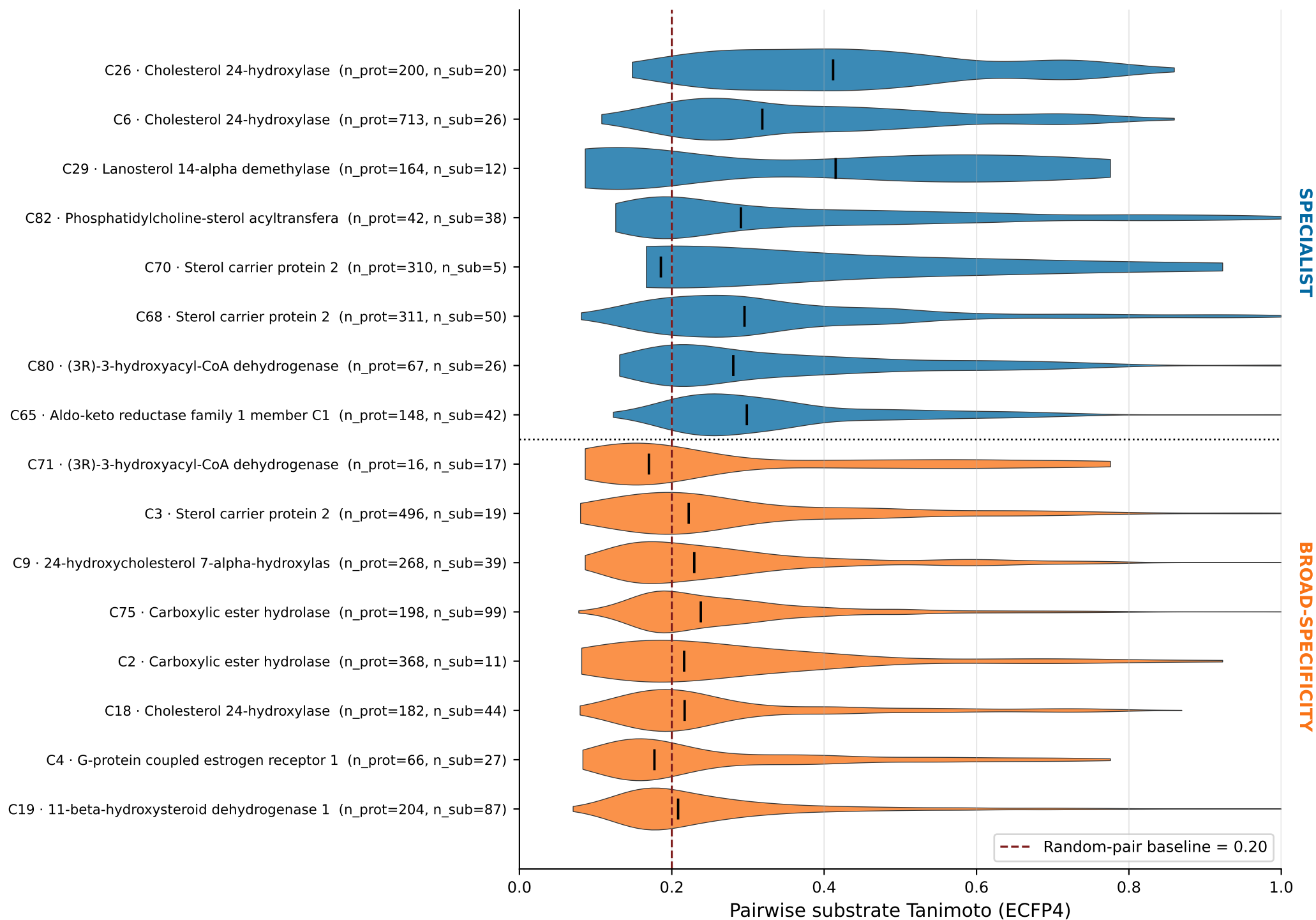
Enzyme clusters — top 8 specialists vs top 8 broad-specificity
