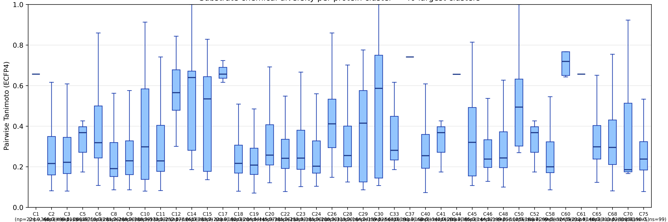
Substrate chemical diversity per protein cluster — 40 largest clusters
