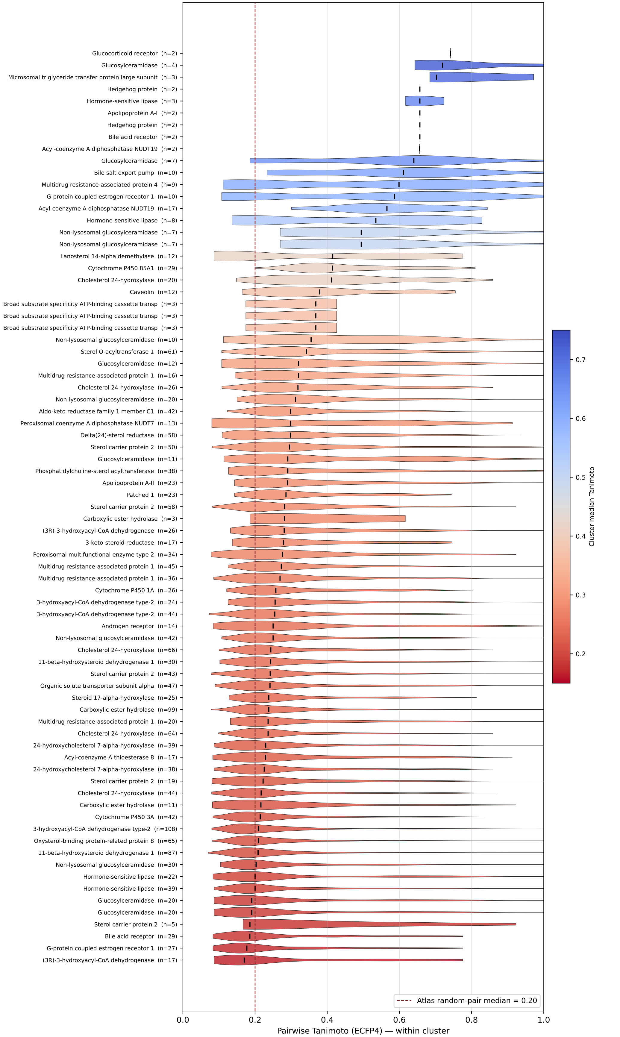
Within-cluster substrate chemical similarity ( 77 of 82 clusters with ≥2 fingerprinted substrates, sorted by median)
