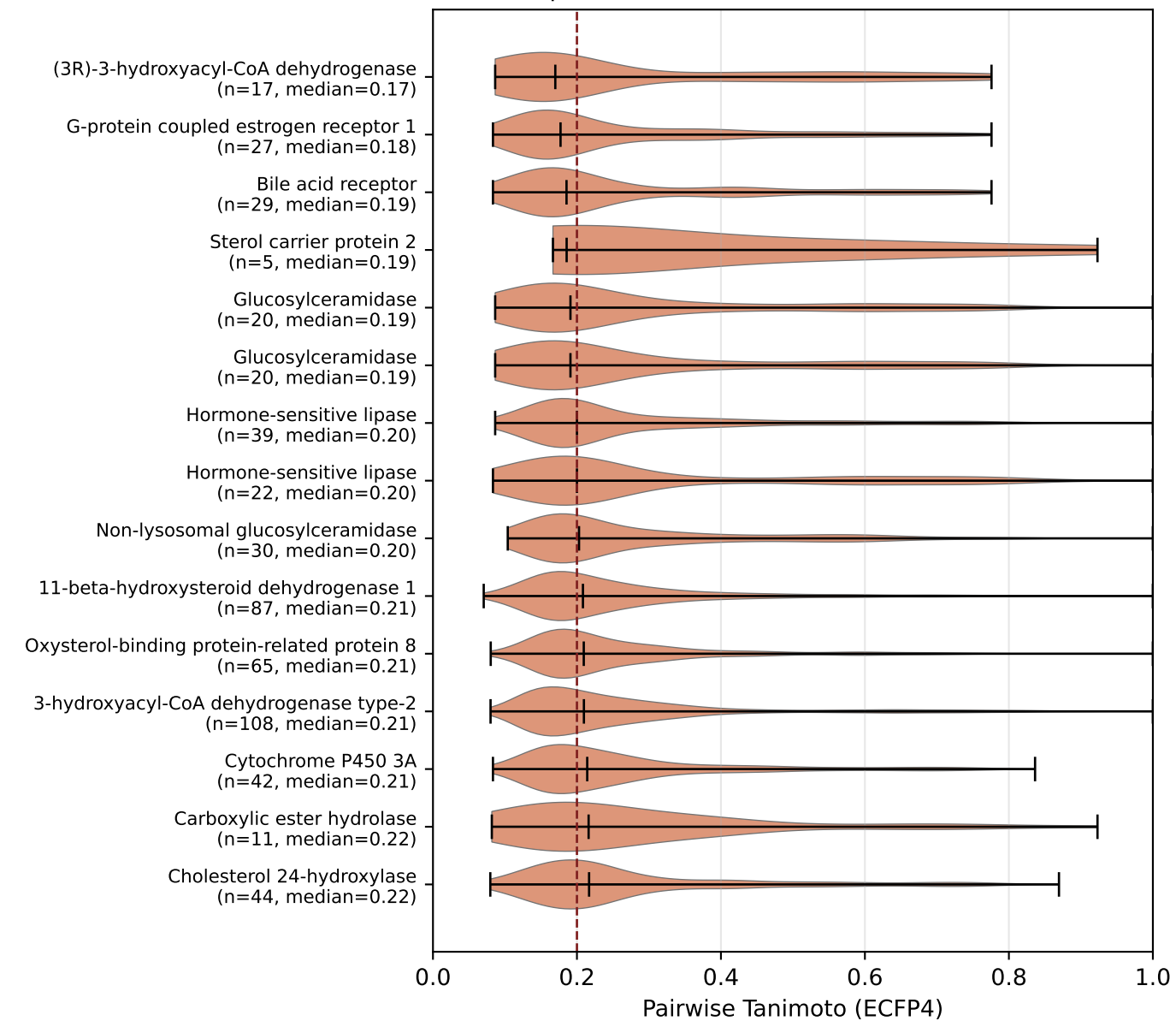
Top 15 most CHEMICALLY DIVERSE clusters
