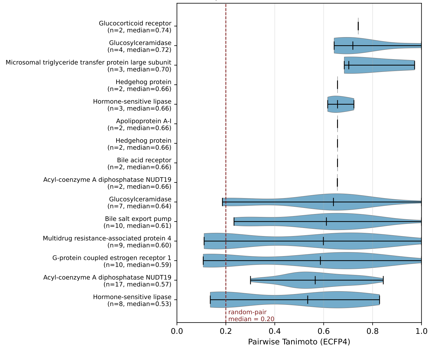
Top 15 most CHEMICALLY UNIFORM clusters
