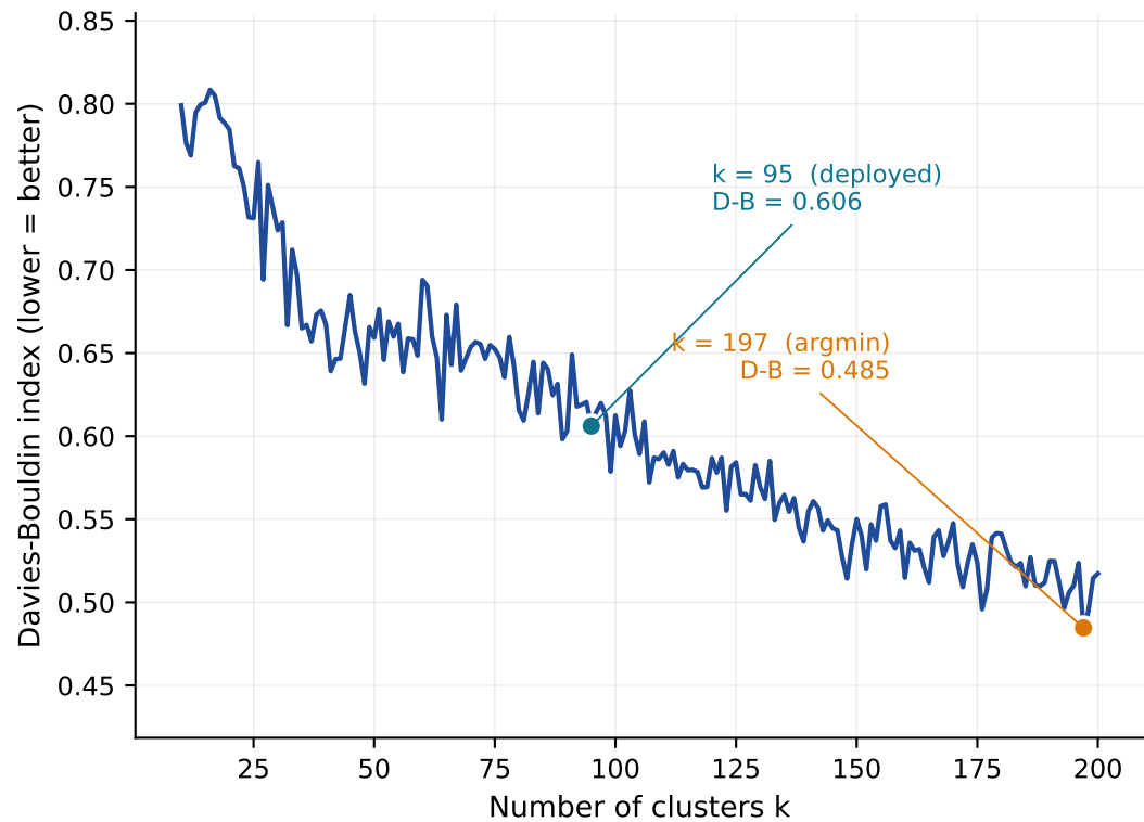
B. Davies-Bouldin
