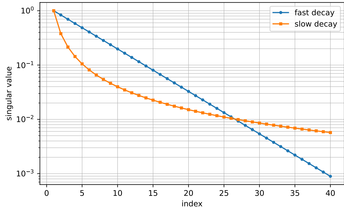
Toy singular value decay
