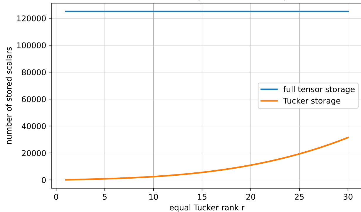
Full tensor storage vs Tucker storage
