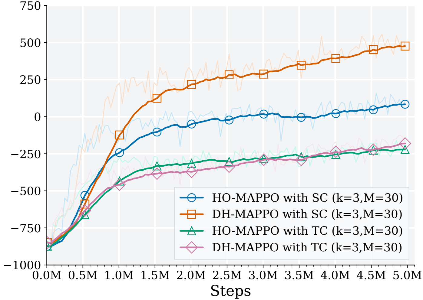
Average episode reward
