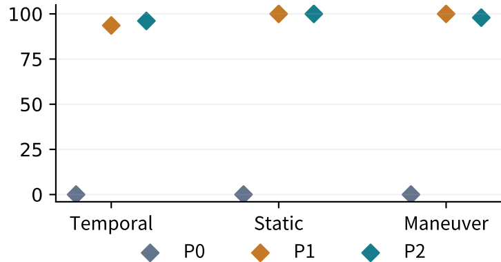
Contract-pair accuracy (%)
