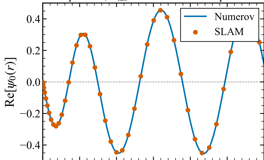
p + {}^{12}\text{C} , E_{\text{lab}} = 30 \text{ MeV} – Real part
