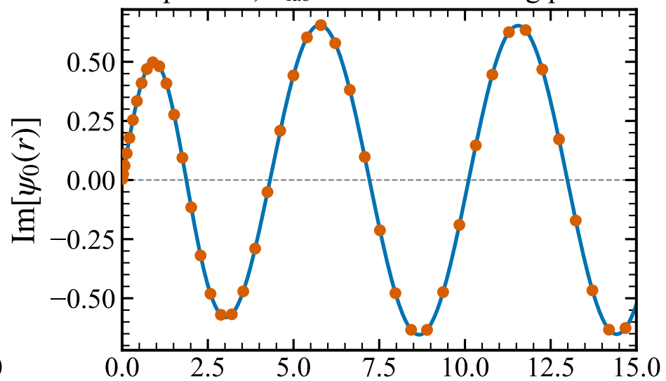
p + {}^{12}\text{C} , E_{\text{lab}} = 30 \text{ MeV} – Imag part
