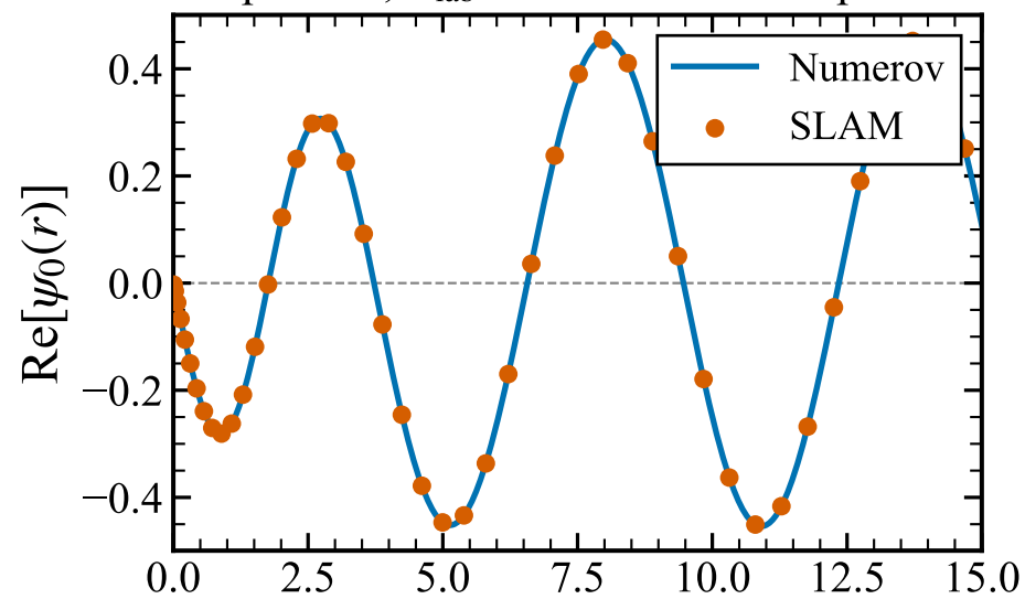
p + {}^{12}\text{C} , E_{\text{lab}} = 30 \text{ MeV} – Real part
