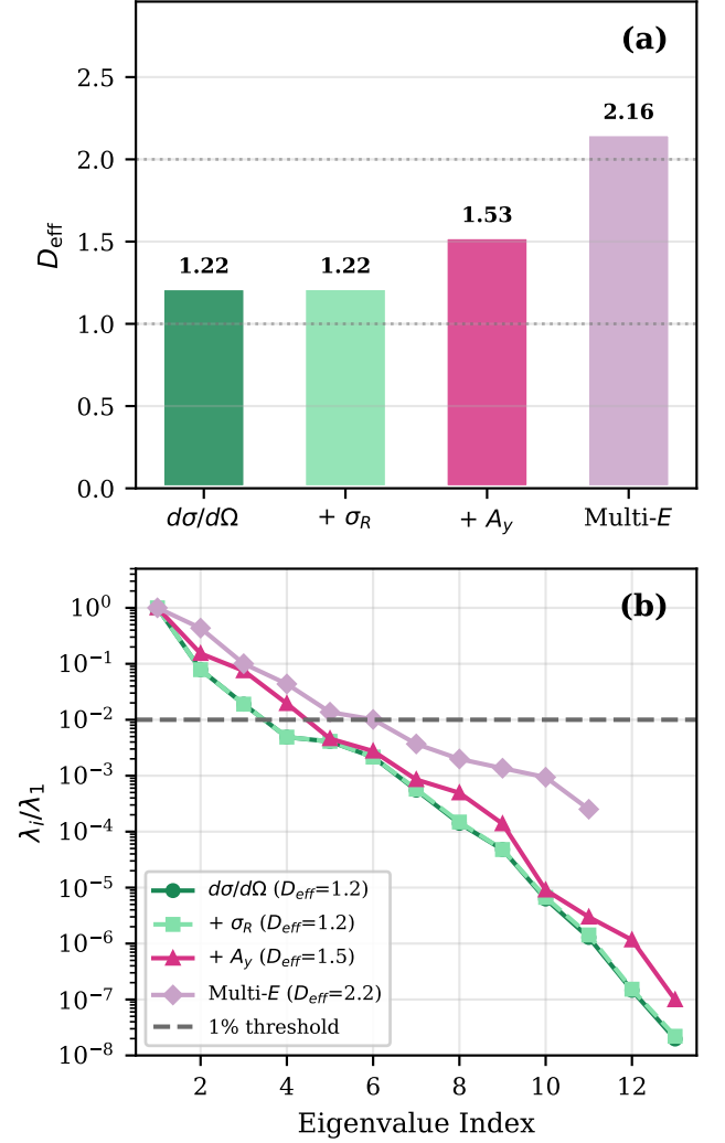
FIG. 3. Step-by-step constraint analysis for n+^{40}\text{Ca} . (a) D_{\text{eff}} for 13 local parameters increases as observables and energies are added (Steps 1–3 at 50 MeV; Step 4 combining 7 energies 10–200 MeV via Jacobian projection through the KD02 universal coefficient space): elastic alone (1.22), +\sigma_R (no change), +A_y (1.53), multi-energy with all observables (2.16). (b) Eigenvalue spectra at each step. The multi-energy curve has 11 non-zero eigenvalues because the KD02 constraints r_w = r_v and a_w = a_v eliminate 2 of the 13 local degrees of freedom.
