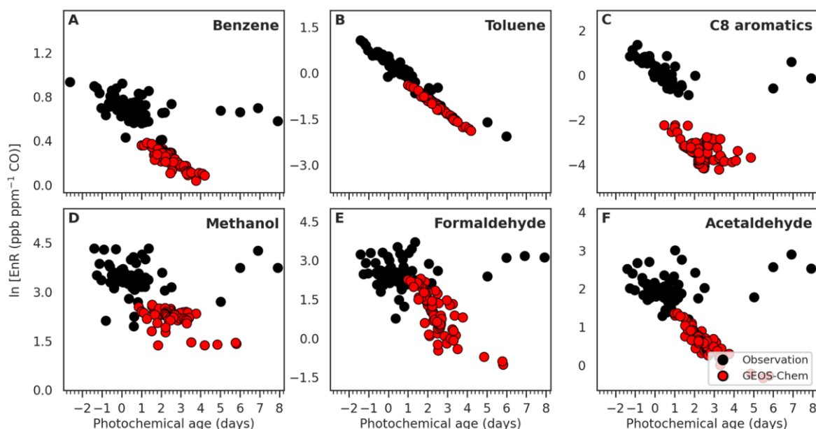
Black points show the ground measurements and red points show GEOS-Chem. Each gas is compared with carbon monoxide, and the horizontal axis represents chemical age. Steeper downward patterns indicate faster removal. Flatter patterns are consistent with continued formation partly offsetting chemical losses, although mixing may also contribute.
