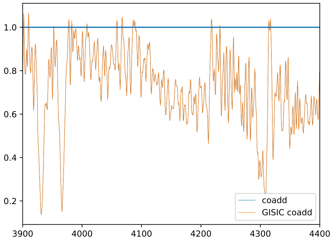
hd198269 coaddition of m1b and m2b
