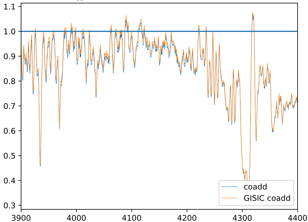
jy1894 coaddition of m1b and m2b
