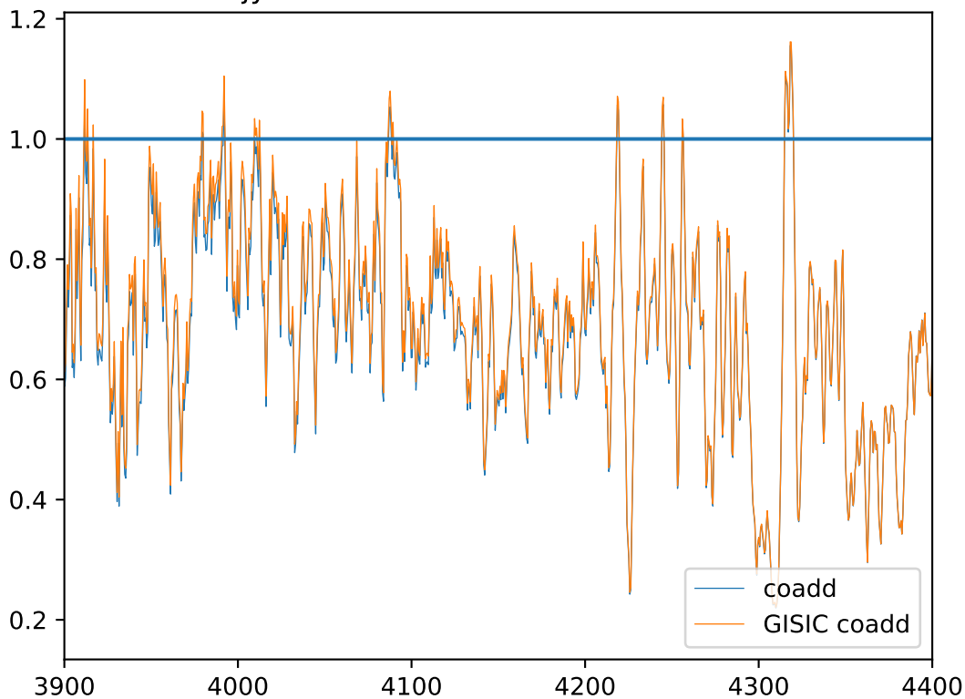
jy1900 coaddition of m1b and m2b
