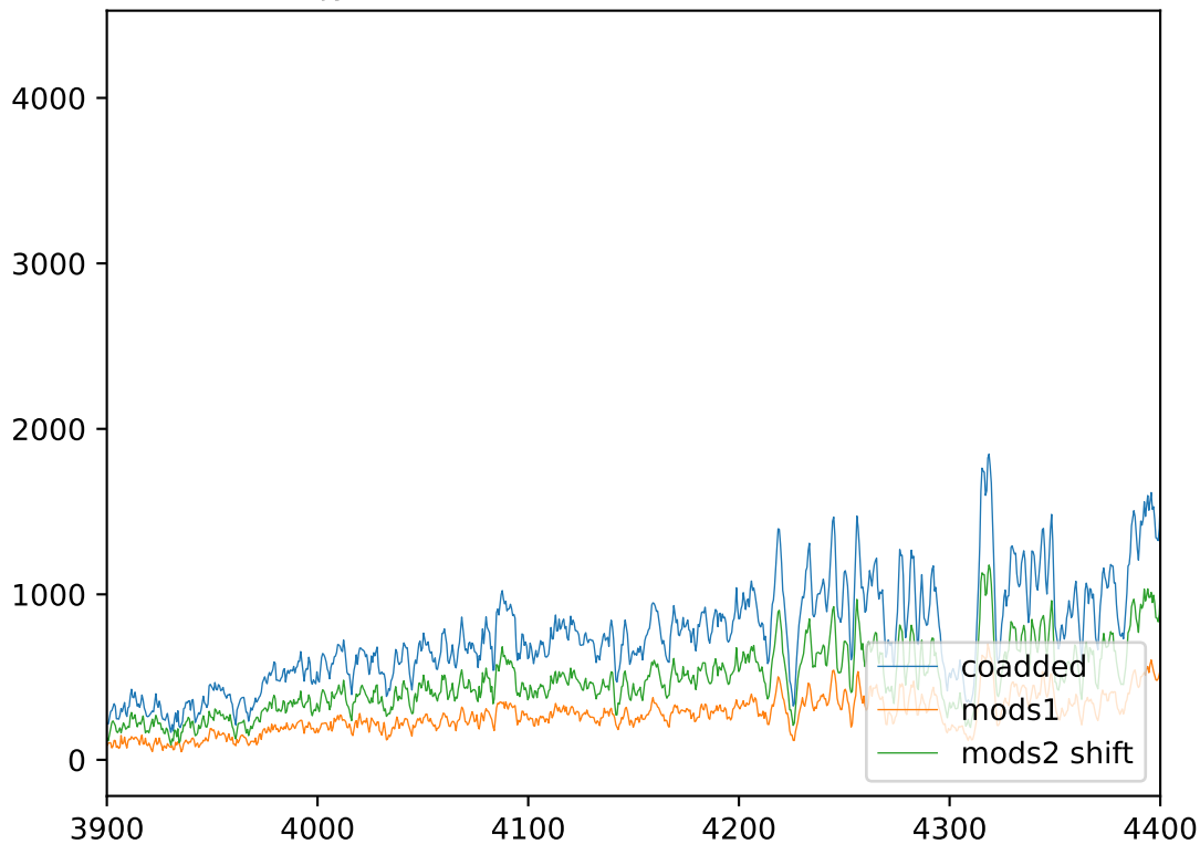
jy1900 coaddition of m1b and m2b
