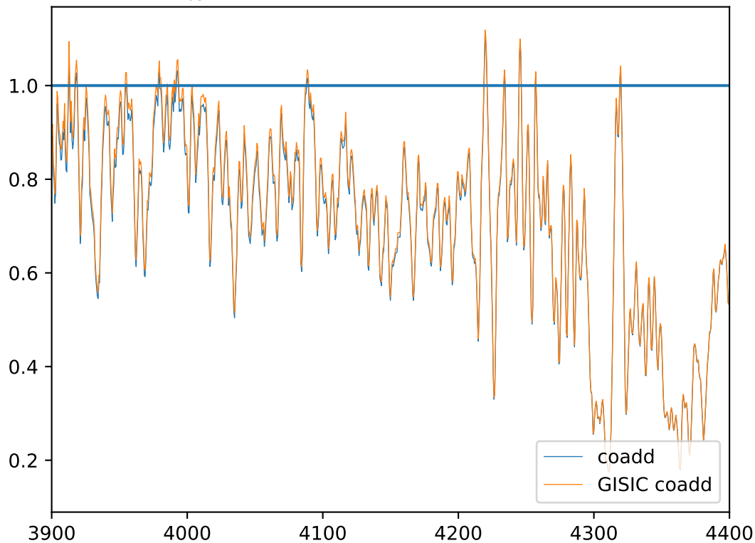
jy1926 coaddition of m1b and m2b
