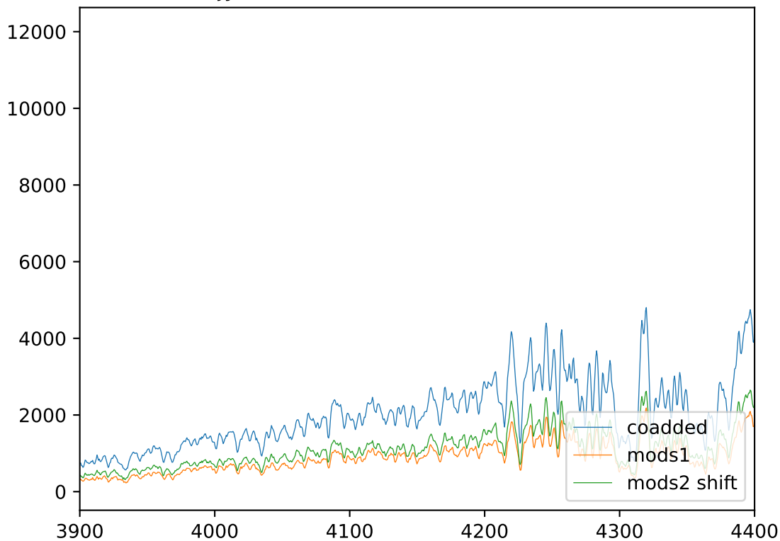
jy1926 coaddition of m1b and m2b
