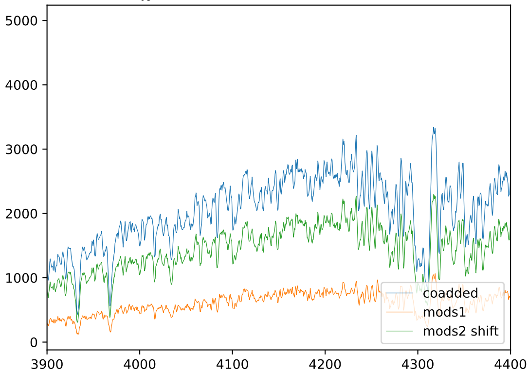
jd2183 coaddition of m1b and m2b
