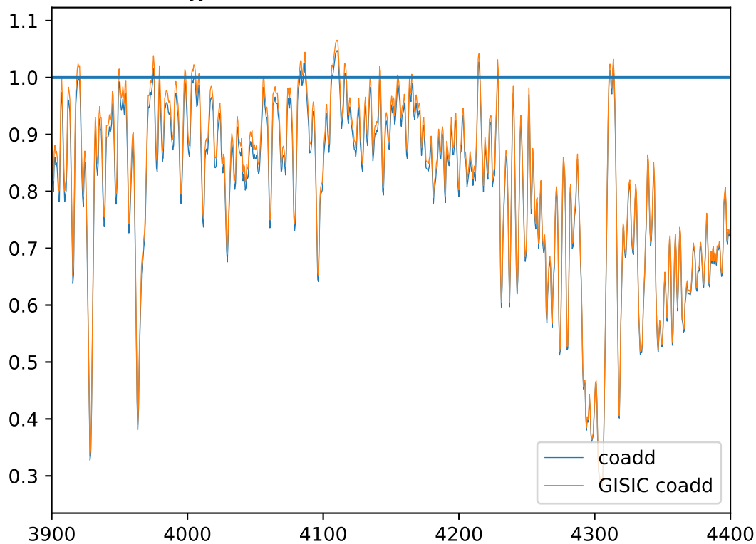
jy2552 coaddition of m1b and m2b
