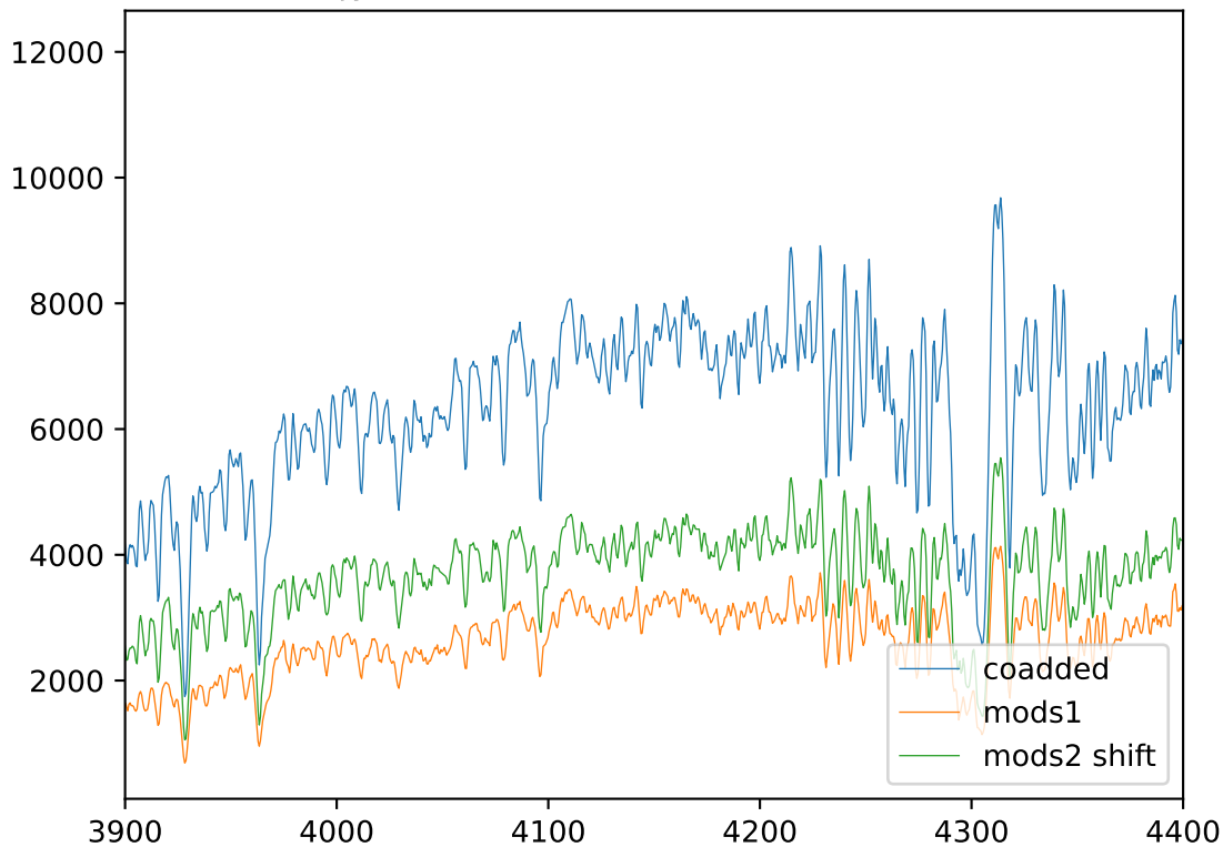
jy2552 coaddition of m1b and m2b
