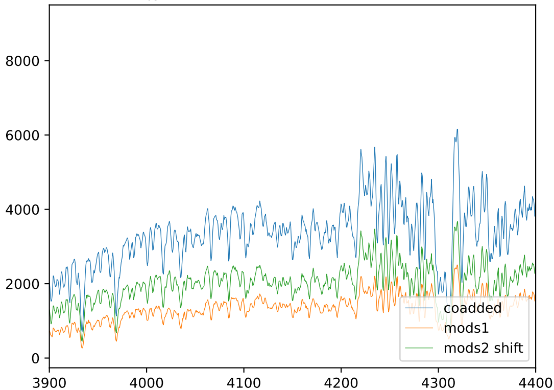
jy2553 coaddition of m1b and m2b
