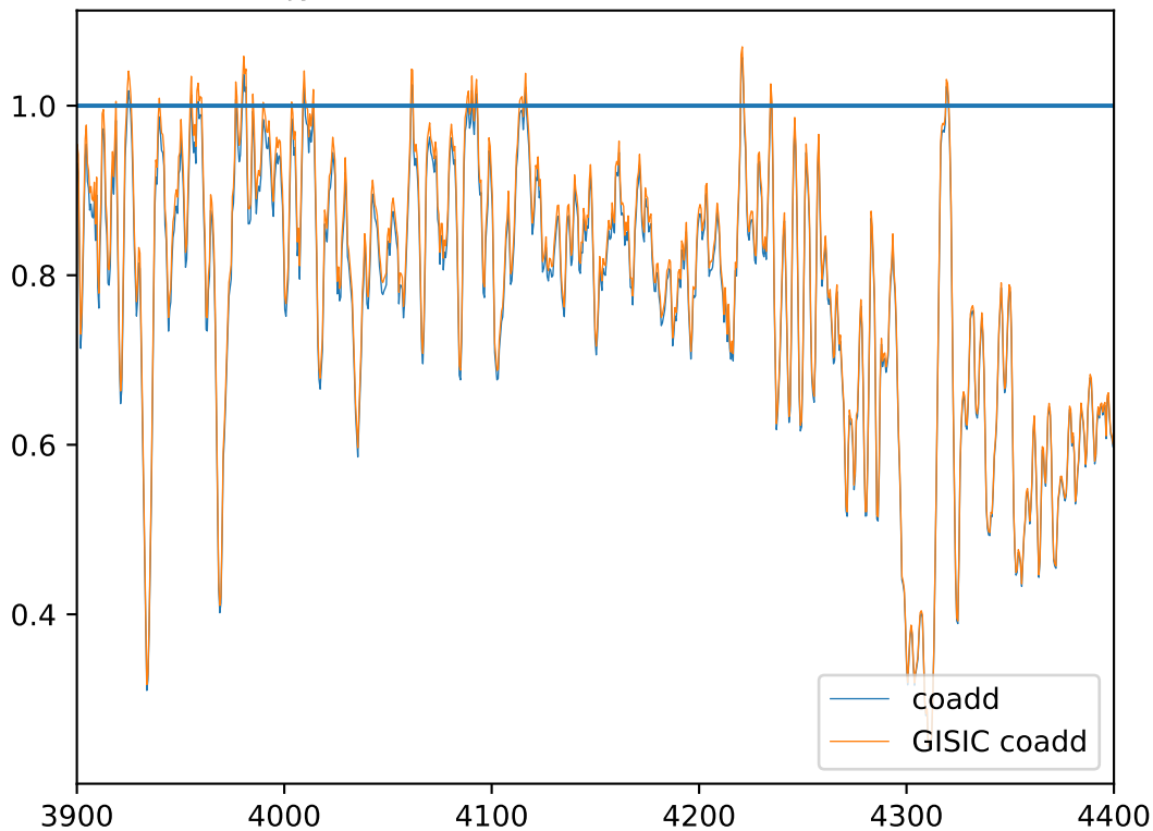
jy2866 coaddition of m1b and m2b
