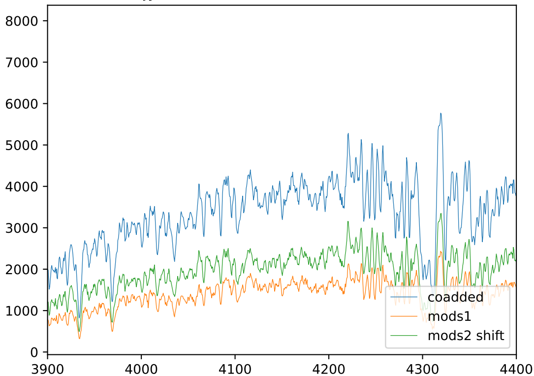
jy2866 coaddition of m1b and m2b
