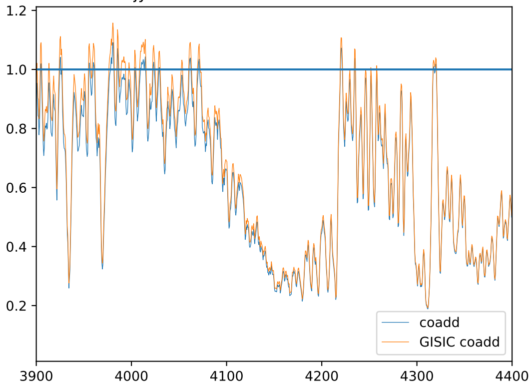
jy3321 coaddition of m1b and m2b
