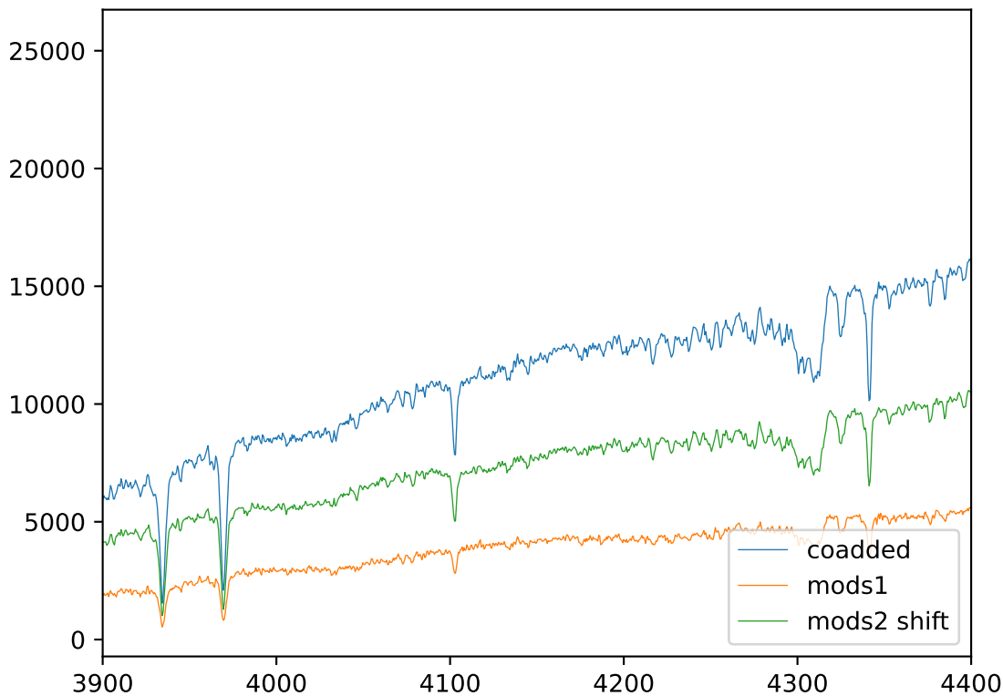
smss1738 coaddition of m1b and m2b
