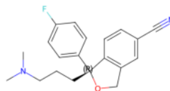
(R)-citalopram (CID 6101829)
