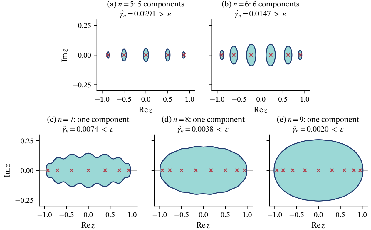
FIGURE 1. Numerically sampled open pseudospectra of A_n(1/4) at \varepsilon = 10^{-2} . Shading marks the sampled pseudospectrum and crosses mark the exact eigenvalues. The samples show component coalescence between n = 6 and n = 7 .
