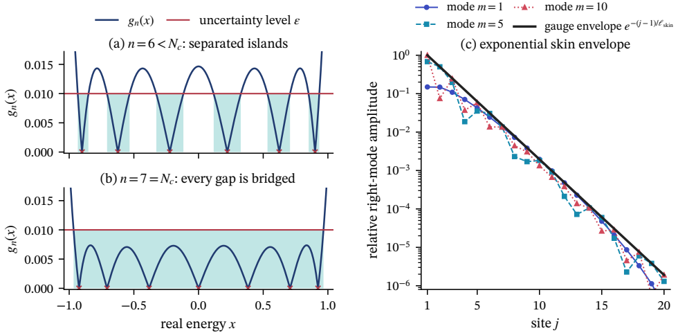
FIG. 3. Why the uncertainty clouds merge, for a = 1/4 and \varepsilon = 10^{-2} . In (a)–(b), the blue curves are g_n(x) = s_{\min}(xI_n - A_n) , the red line is the perturbation budget, and the teal portions are the real pseudospectrum. At n = 6 , peaks above the budget separate the six eigenvalue islands; at n = 7 = N_c , every inter-eigenvalue location lies below the budget and the real trace is one interval. Panel (c) shows the common exponential envelope of right skin modes at n = 20 . Its amplitude decay length is \ell_{\text{skin}} = 2/\log(1/a) , the coefficient in the asymptotic law for N_c . Reversing the site convention reverses the edge but not the merger criterion.
