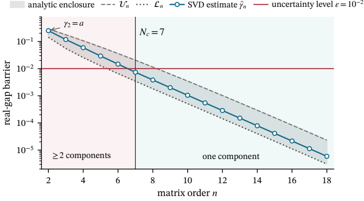
FIG. 2. Finite-size crossing of the perturbation budget. Gapwise float64 SVD estimates \hat{\gamma}_n of the strictly decreasing barriers and the exact analytic enclosure \mathcal{L}_n(a) \leq \gamma_n \leq \mathcal{U}_n(a) for a = 1/4 . The plotted estimates first cross below \varepsilon = 10^{-2} at n = 7 , again indicating the reported numerical threshold. Independently, the exact analytic bounds in (2.4) give 6 \leq N_c \leq 9 . To the left of the crossing at least one component separator survives; from the crossing onward there is one component. The nearly parallel log-scale curves display the common (n+1)a^{n/2} scale.
