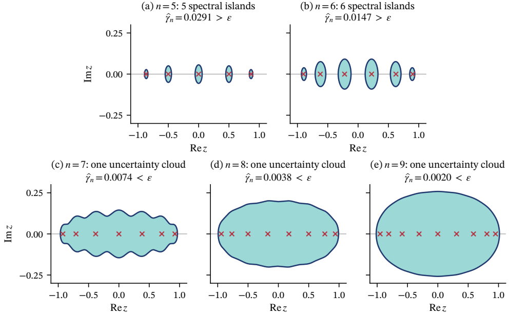
FIG. 1. Topology change indicated by the float64 computation at a = 1/4 and \epsilon = 10^{-2} . Shading depicts \{z : s_{\min}(zI_n - A_n) < \epsilon\} , and crosses are open-boundary eigenvalues. Gapwise SVD estimates give (\hat{\gamma}_5, \dots, \hat{\gamma}_9) = (0.02909836, 0.01465829, 0.007364219, 0.003820033, 0.001992747) . Applying the grid/Lipschitz check to the float64 samples places the computed margins for n = 5, 6 above \epsilon and those for n = 7, 8, 9 below it, yielding the reported numerical threshold N_c = 7 . As explained in the text, these checks are not interval certificates. In the two displayed pre-threshold cases every component contains one eigenvalue, so the components are mode-resolved uncertainty islands. At n = 7 the last separator is lost and all eigenvalues belong to one uncertainty cloud. The merger is a perturbation-level-dependent pseudospectral event, not the onset of skin localization.
