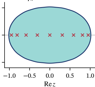
(e) n=9 : connected \hat{\gamma}_n=0.0020 < \varepsilon
