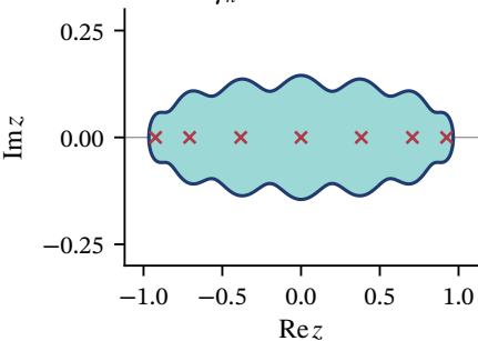
(c) n=7 : connected \hat{\gamma}_n=0.0074 < \varepsilon
