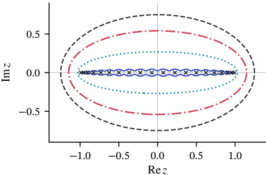
(a) OBC pseudospectra and PBC symbol
