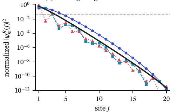
(b) OBC right-eigenvector skin modes
