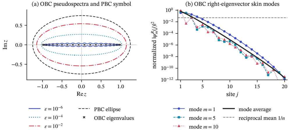
FIG. 3. Hatano–Nelson interpretation for a = 1/4 and n = 20 . (a) The open-boundary eigenvalues lie in the real segment [-2\sqrt{a}, 2\sqrt{a}] , whereas the periodic symbol e^{ik} + ae^{-ik} traces an ellipse. The nested contours are boundaries of strict pseudospectra. (b) Right eigenvectors \psi_m^R(j) \propto a^{(j-1)/2} \sin \frac{m\pi j}{n+1} accumulate at the left edge. Reversing the site convention reverses the edge but not the pseudospectral conclusions.
