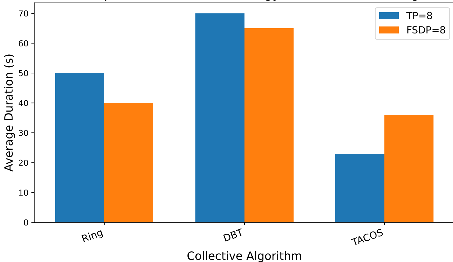
[Cartoon Graph] Parallelization Strategy across AllReduce Algorithm
