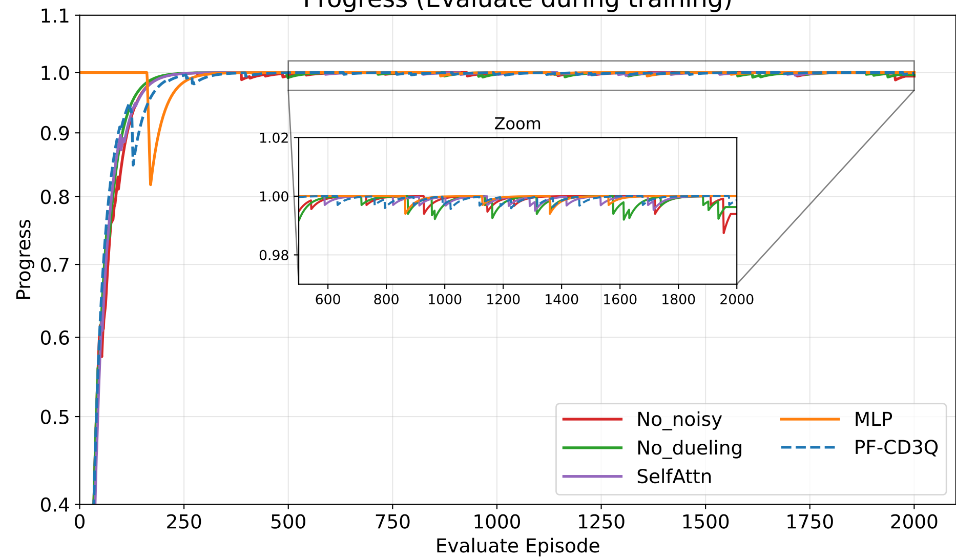
Progress (Evaluate during training)
