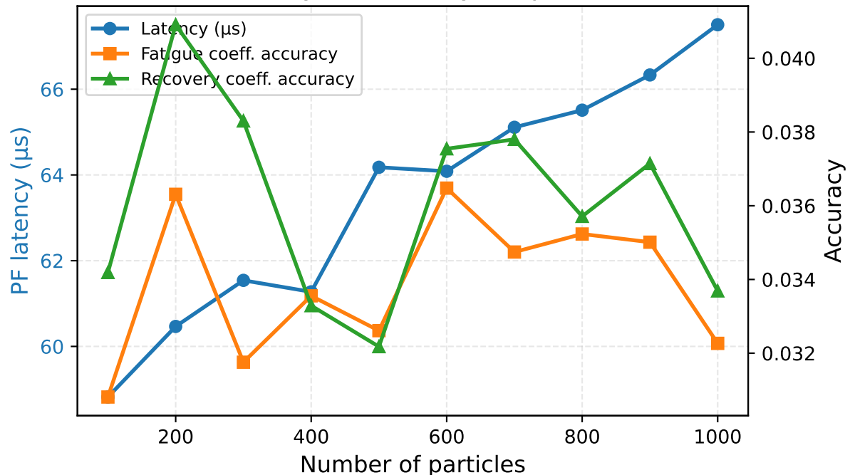
PF latency &amp; accuracy vs. particles
