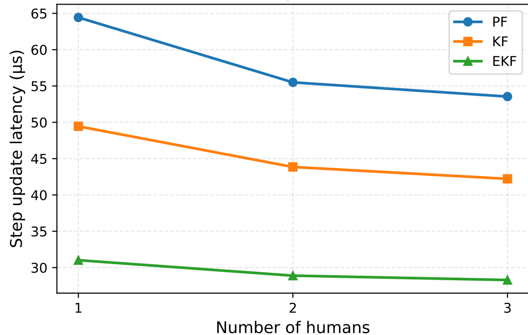
Filter latency vs. humans
