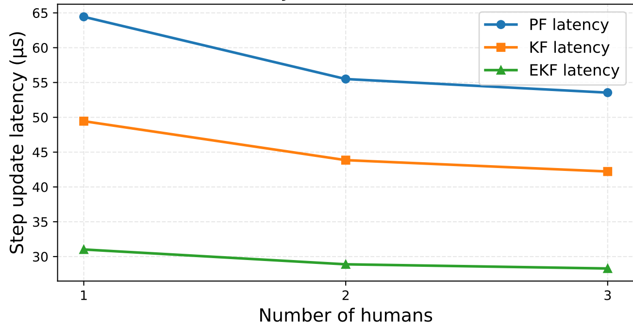
Filter latency vs. number of humans
