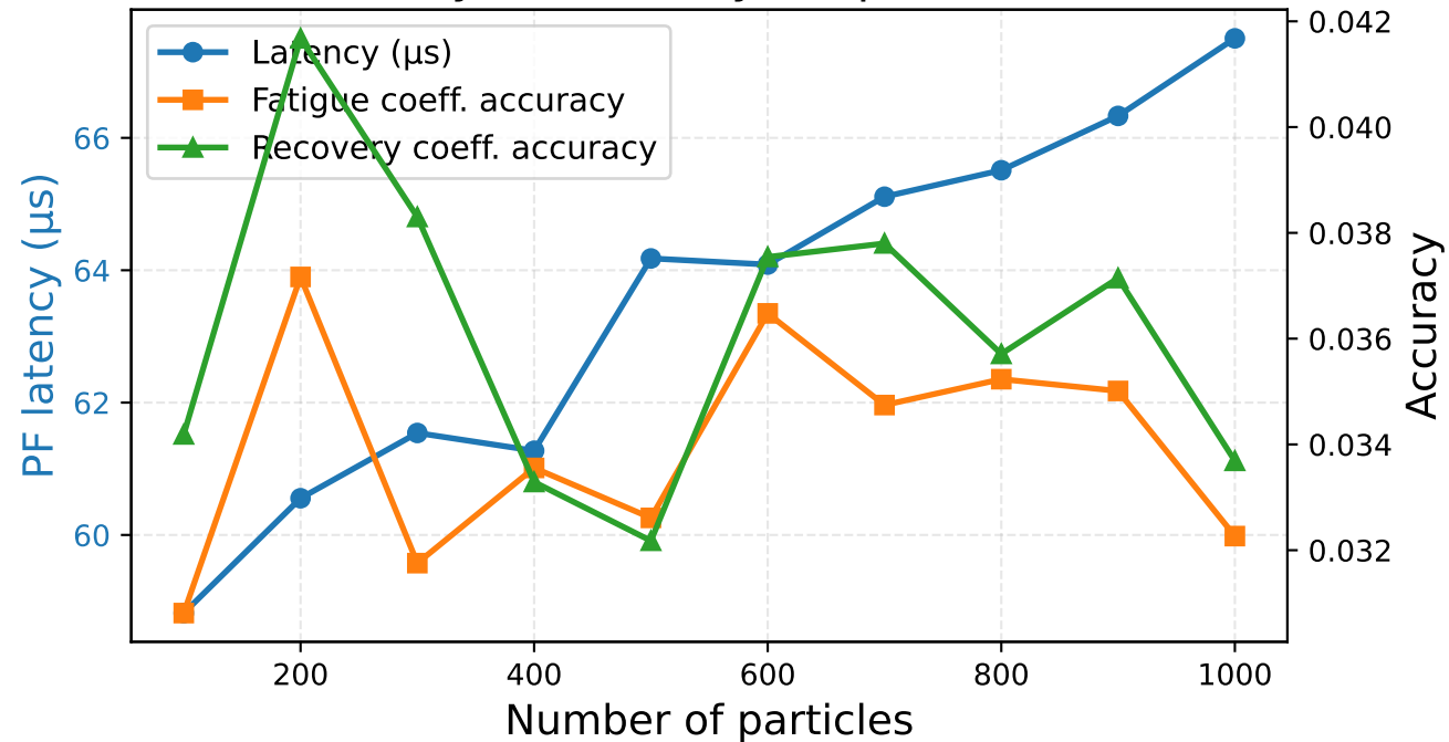
PF latency & accuracy vs. particle count
