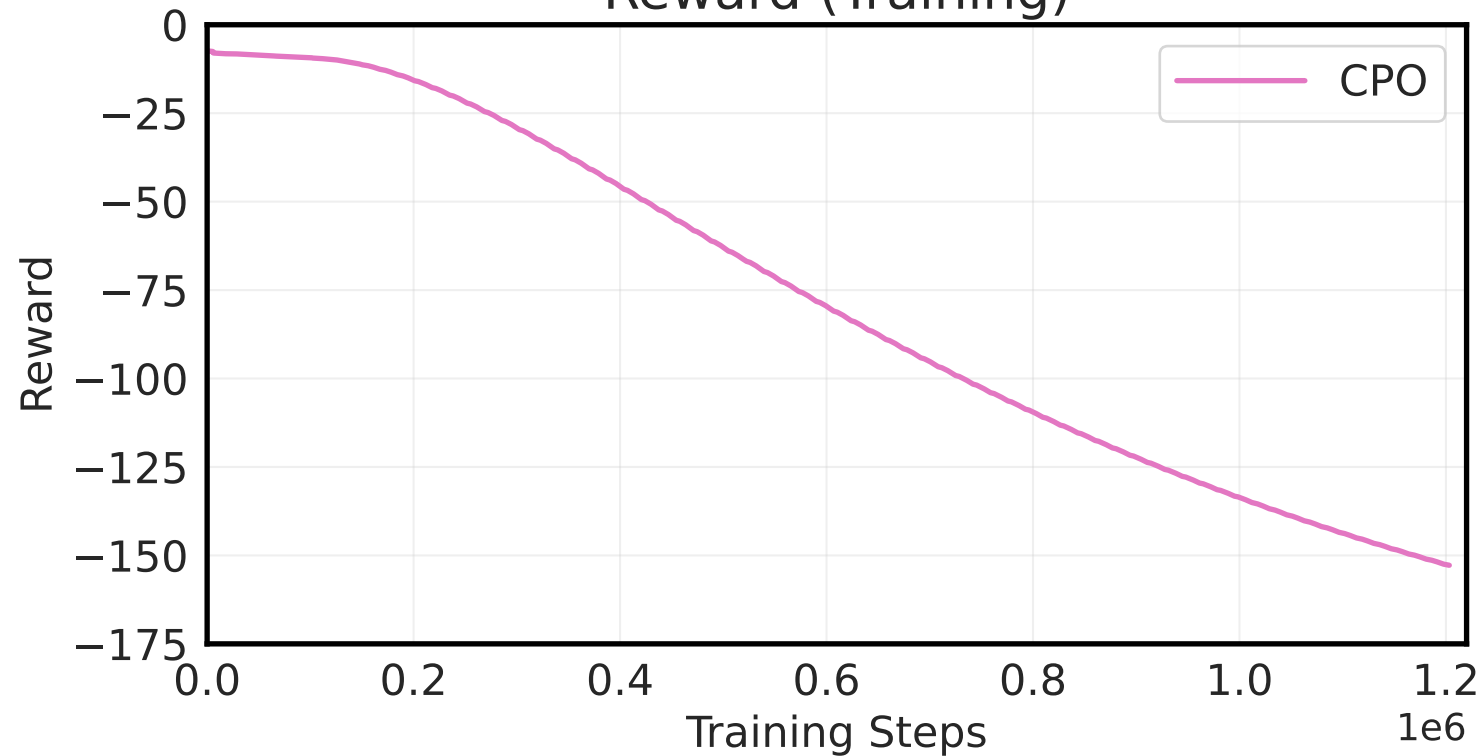
Reward (Training)
