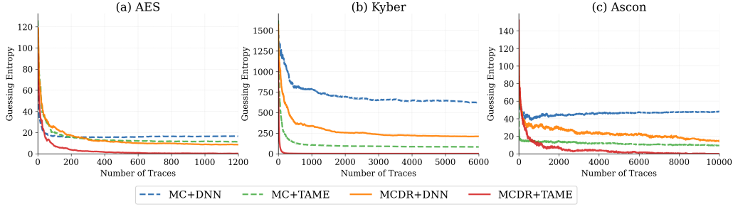
Figure 3: DNN vs TAME: GE evolution comparing DNN and TAME frameworks under two labeling methods on AES, Kyber, and ASCON datasets.
