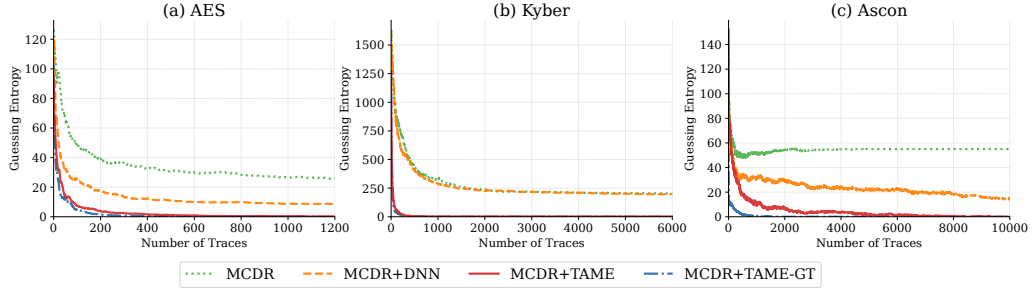
Figure 5: GE evolution comparing gaps between semi-supervised TAME-GT and blind frameworks under MCDR labeling method.
