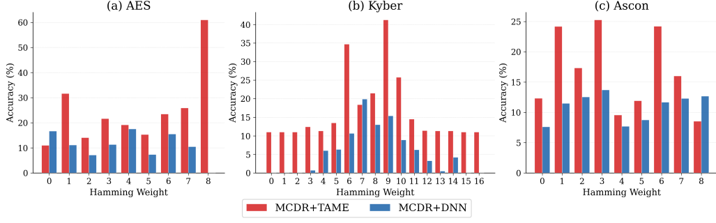
Figure 4: Label accuracy on the attack set under DNN and TAME framework on AES, Kyber, and ASCON datasets.
