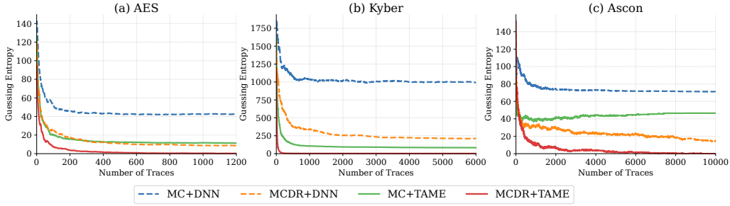
Figure 2: MC vs MCDR: GE evolution comparing MC and MCDR labeling methods under DNN and TAME frameworks on AES, Kyber, and ASCON datasets.
