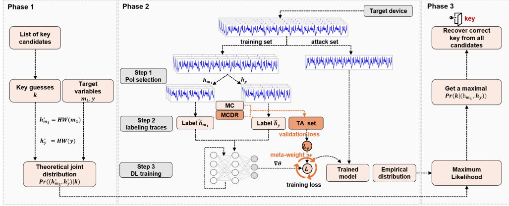
Figure 1: Analysis framework of DL-BSCA. Spanish orange blocks denote components proposed in this work: MCDR labeling (Section 3.3), TA selection (Section 3.2.1), and Meta-weight Estimation (Section 3.2.2). Light orange blocks denote existing components from prior work [LDLL14, CR17, RYJ + 25]: Phase 1 pre-computation, PoI selection, standard DNN training, and Phase 3 distribution comparison.
