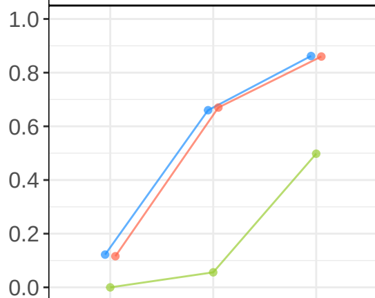
WI, c = 0.5
