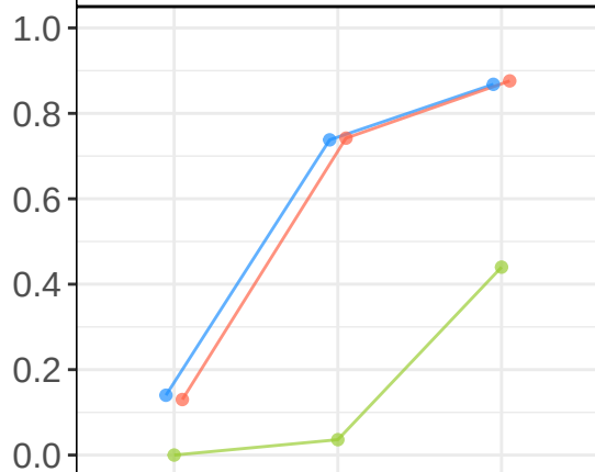
WD, c = 0.5
