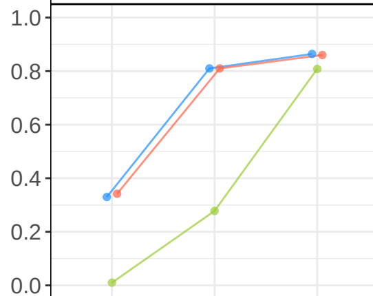
Bat, c = 0.5
